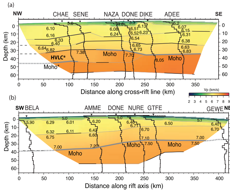
Figure 7. Comparison of joint inversion shear wave velocity results ( V_s ) for stations located near active source profiles with active source 2-D modeling results ( V_p ) from Maguire et al. [2006]. (a) Comparison to cross-rift line. (b) Comparison to along-axis line. The depth to major boundaries, such as the Moho and intracrustal reflectors, matches closely between the two sets of results. Numbers on the profiles are modeled V_p velocities from active source modeling. Because of the uncertainty in converting from V_s to V_p (or vice versa) with only whole-crustal V_p/V_s ratios available from independent analyses [ Dugda et al. , 2005; Stuart et al. , 2006], we have not tried to compare absolute velocity. The HVLC (high-velocity lower crust) modeled in the active source profile along line 1 in Figure 7a is not a feature characteristic of the NW shoulder and is spatially very localized (Figure 8). The depth to Moho beneath the NW shoulder is \sim 40 km [from Stuart et al. , 2006; Dugda et al. , 2005; this study]. Accordingly, we refer to the HVLC body and the Moho as observed on the wide-angle profile beneath the NW shoulder as HVLC* and as Moho*.
