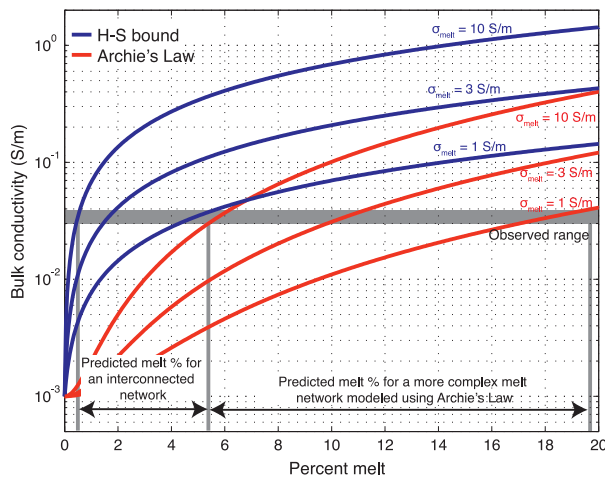
Figure 15. Constraints on the amount of melt present in the lower crust in Ethiopia from observed conductivity values of Whaler and Hautot [2006]. Blue curves are calculated using the upper Hashin-Shtrikman bounds, which assumes a connected melt network and provides a lower bound on the amount of melt present. Red curves are calculated using the modified version of Archie's Law for materials containing partial melt [ Hermance , 1979] for a matrix conductivity of 0.001 S/m and melt conductivities of 1, 3, and 10 S/m. Between 0.5% and 5% melt is present in the lower crust using the H-S upper bound, and between 6% and 20% melt is present using the modified form of Archie's Law.
