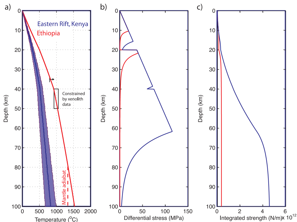
Figure 18. (a) Geotherms, (b) strength profiles, and (c) integrated strength of the lithosphere adjacent to the eastern branch of the East African Rift System (blue curves) and adjacent to the Main Ethiopian Rift (red curves) beneath the Ethiopian Plateau. In Figure 18a a range of temperature with depth is shown for the Eastern Rift; the central curve is used for the plots in Figures 18b and 18c. The integrated strength of the lithosphere (Figure 18c) surrounding the eastern branch is an order of magnitude higher than surrounding the Main Ethiopian Rift. See Table 2 for values used in the calculations of the geotherms (Figure 18a) and strength envelopes (Figures 18b and 18c). All values used for the Ethiopia and Kenya curves were the same with the exception of the surface heat flow, the range for which was taken from Nyblade et al. [1990] for Kenya and modeled using subsurface estimates of temperature for Ethiopia based on the xenolith data from Conticelli et al. [1999] as a constraint. In Figure 18a the vertical line and accompanying arrow in the lower crust for the Ethiopian curve indicate the temperature at which the shear modulus drops sharply [Kampfmann and Berckhemer, 1985] and dV_s/dT increases. Our analysis indicates that the most likely cause for the observed low lower crustal shear wave velocity below 35 km is temperature, and therefore we are at or above this temperature in the lower crust in Ethiopia.
