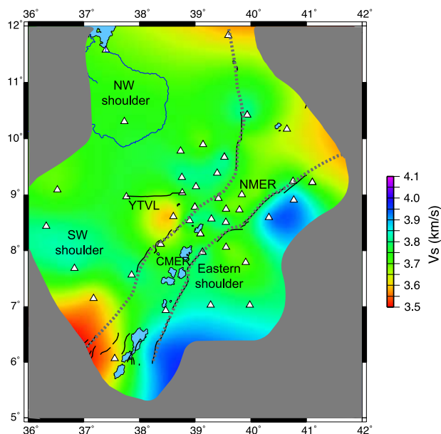
Figure 12. Contour map of lowermost (average of the lower 5 km) crustal shear wave velocity from our joint inversion results. Symbols as in Figure 10. The shear wave velocity of the lower crust in our study area is 3.6–3.8 km/s across nearly the entire region, with only two stations in the study area having a lower crustal velocity of 3.9 km/s. The shear wave velocity of the lower crust along-strike in the Mozambique Belt to the south is 3.9–4.1 km/s [Julia et al. , 2005].
