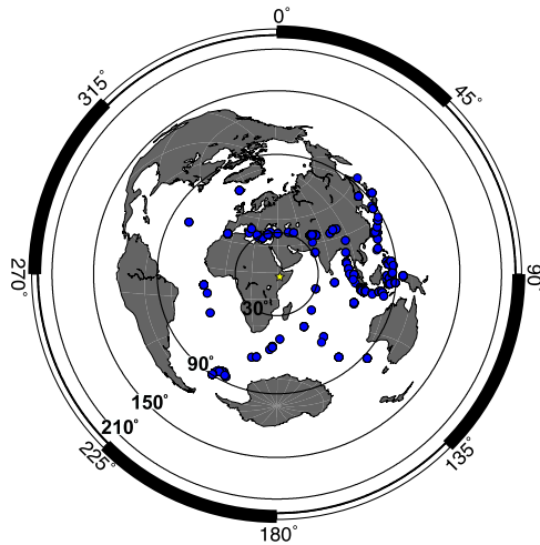
Figure 3. Distribution of earthquakes used for receiver function analysis. 148 earthquakes with M_w > 5.5 at offsets of 30^\circ to 95^\circ were used. The yellow star represents the location of the center of our study.
