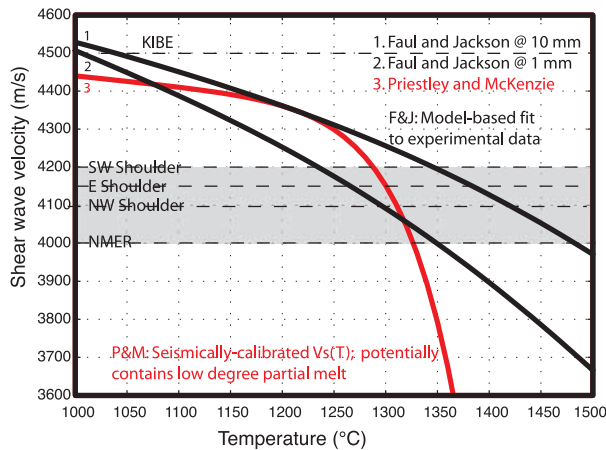
Figure 13. Estimated shear wave velocity versus temperature in the upper mantle from Faul and Jackson [2005] and Priestley and McKenzie [2006]. The two curves from the Faul and Jackson [2005] model are for upper mantle grain sizes of 1 and 10 mm. The gray box represents the range of shear wave velocity values observed beneath the MER and the adjacent plateaus. The horizontal dashed black lines show the average upper mantle temperature for the different regions discussed in the text. For comparison, the upper mantle temperature at KIBE is \sim 4.5 km/s, which corresponds to a temperature much less than 1000^\circ\text{C} for the Priestley and McKenzie [2006] model, which may be the more accurate of the two curves in this temperature range given that the Faul and Jackson [2005] model is only calibrated for temperatures between 1000^\circ\text{C} and 1300^\circ\text{C} . The two models show different behavior, but for a velocity of 4.1 km/s both predict an upper mantle temperature of \sim 1300^\circ\text{C} .
