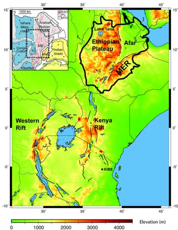
Figure 1. Map of East African Rift System. The heavy black line outlines the Ethiopian flood basalt province [from Mohr , 1983]. Lake Tana is the site of off-rift Quaternary volcanism and Oligocene and Quaternary xenoliths [ Conticelli et al. , 1999]. The inset map shows the outline of Figure 1 (heavy dashed box) with respect to the cratons/shields and orogens forming East (yellow) and West (blue) Gondwana (modified from Meert and Lieberman [2008]). EAO, East African Orogen; MTO, Mesozoic-Tertiary Orogen; PC, Precambrian Shield; MB: Mozambique Belt; TC, Tanzanian Craton.
