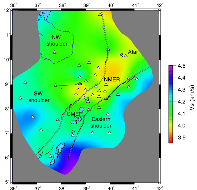
Figure 11. Contour map of uppermost (average of the top 5 km) mantle shear wave velocity from our joint inversion results. Symbols as in Figure 10. The SW shoulder has the highest observed upper mantle V_s within our study area (4.2–4.3 km/s), the eastern and NW shoulder have velocities of 4.0–4.2 km/s, and the NMER/YTVL has the lowest upper mantle velocity, 4.0 km/s. Uppermost mantle velocity in the PREM model is 4.5 km/s.
