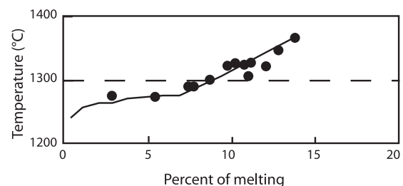
Figure 14. Experimental results for percent melt versus temperature for depleted peridotite, modified from Hirschmann et al. [1998] by permission of Oxford University Press. At 1300^\circ\text{C} (our upper bound on temperature if the low upper mantle shear wave velocity below Ethiopia is caused only by high temperature), melt percent would be over 5% on the basis of these experimental results. Black circles are reported measurements, and the solid black line is the predicted curve using the MELTS algorithm.
