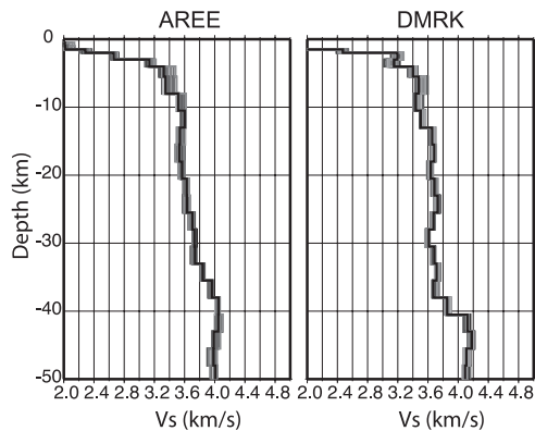
Figure 6. Results of bootstrap inversions at stations AREE (within the Northern MER) and DMRK (on the NW shoulder). The inversions test the sensitivity of the method to variations in inversion parameters, including 12 distinct starting models with varying velocity and Poisson's ratio, different groups of input data, and three different weighting parameters between receiver functions and surface waves (see text). The tight clustering of the output inversions in the lower crust shows the low sensitivity of the inversion to these parameters. The greater spread in the output models in the upper crust (above 10 km) may represent greater heterogeneity in the upper crust, as different groups of receiver functions include receiver functions from different events which travel different paths and therefore sample different geologic features. The low sensitivity of the inversions to the weighting parameter between receiver functions and surface waves indicates that while the surface wave data provide a smooth velocity function, the receiver functions provide most of the structure in the output inversion. The color of the line represents the RMS fit of that model to the data, with the black line providing the best RMS fit and lighter shades of gray progressively worse.
