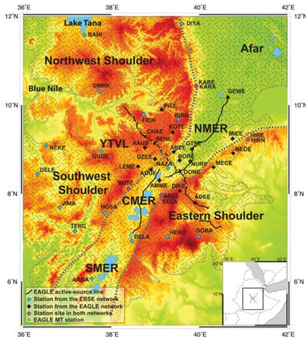
Figure 2. Map of the Main Ethiopian Rift showing broadband stations (diamonds), EAGLE active source profiles (continuous black lines), the EAGLE MT stations (yellow circles), and the distribution of flood basalts (cross hatching) [from Mohr, 1983 ]. Indentations into the flood basalt distribution in this region are largely erosional (e.g., the gorge of the Blue Nile), but flood basalts pinch out to the SE. The dashed gray lines outline the structural rift valley. Stations used in our joint inversion are labeled; stations with two names were colocated in the EAGLE and EBSE networks. YTVL, Yerer-Tullu Wellel Volcano-tectonic Lineament, an ~E-W trending zone separating the NW and SW shoulders [Keranen and Klempner, 2008]. The inset map shows the location of the active source profiles in the Horn of Africa.
