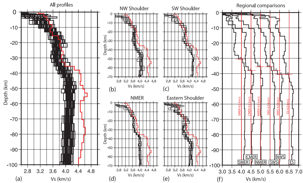
Figure 9. Profiles of our joint inversion results. (a–e) The red profile is the joint inversion result for KIBE [Julia et al. , 2005], a station located along-strike in the Mozambique Belt in Tanzania (location shown in Figure 1). The profile from KIBE is representative of the shear wave velocity structure of the lithosphere surrounding the EARS to the south. (f) A comparison of representative curves from each region with the Moho identified with a horizontal red bar. The curves are offset along the horizontal axis for plotting purposes; the vertical red bars identify the 4.0 km/s line for each profile.
