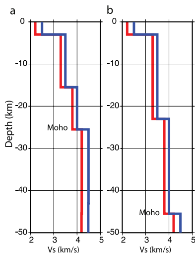
Figure 4. Initial models used in the inversion at each station. (a) Two initial velocity profiles with a 25-km crustal thickness. (b) Two initial velocity profiles with a 45-km crustal thickness. These low and high values for crustal thickness bound the range observed previously in the study area. Values of Poisson's ratio of 0.27, 0.29, and 0.31 were used for each of the four displayed curves, resulting in a total of 12 initial velocity models at each station.
