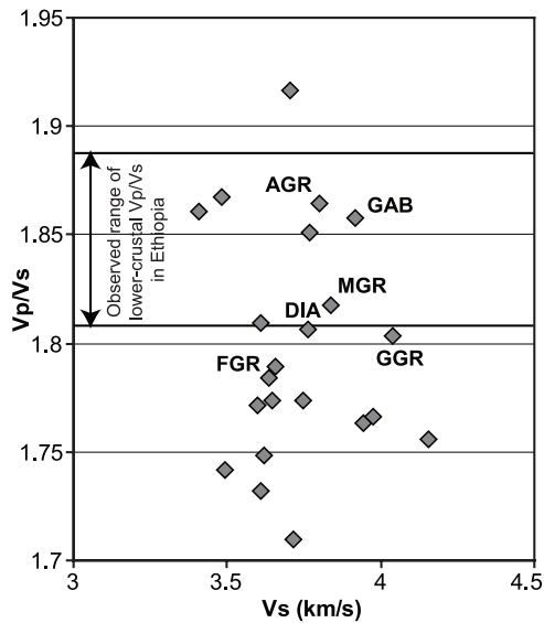
Figure 16. Vp/Vs ratio versus Vs (km/s) at room temperature and 800 MPa for different rock types using data from Christensen [1996]. Vs as shown is higher than expected in the lower crust since data are not temperature-corrected, but Vp/Vs has little dependence on temperature. MGR, mafic granulite; DIA, diabase; GGR, mafic garnet granulite; FGR, felsic granulite; GAB, gabbro. The range of observed lower crustal Vp/Vs values in Ethiopia, calculated using our joint inversion results for Vs and active source Vp profiles, is shown by the horizontal black lines. The Vp/Vs ratio of felsic granulite is lower than the range of observed values in Ethiopia. The Vp/Vs ratio of mafic granulite, present in the lower crust both to the north in the Arabian Shield and to the south in Tanzania, lies within the observed range.
