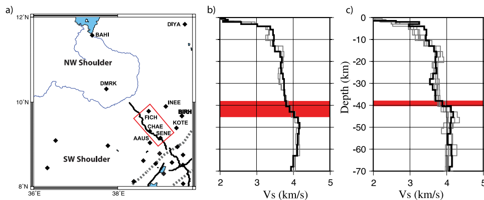
Figure 8. (a) Map of stations on the NW shoulder. Unnamed stations are south of the YTVL on the SW shoulder. (b) Profiles from the NW shoulder at the stations within the red rectangle in Figure 8a, an area on the NW shoulder with an anomalous lower crustal velocity gradient rather than a sharp Moho. (c) Shear wave velocity profiles from the NW shoulder at named stations outside of the red rectangle in Figure 8a, showing a sharp Moho boundary at \sim 40 km.
