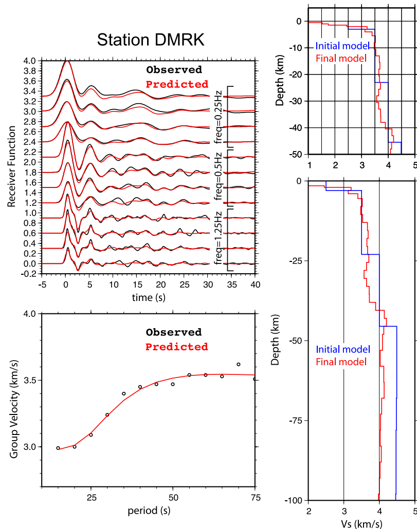
Figure 5. Representative results showing input receiver functions and dispersion curve (black) and synthetic fits from the final model (red). Receiver functions are offset along the vertical axis for plotting purposes. The receiver functions consist of three frequency bands (bracketed), with the four ray parameter groups for each frequency band plotted from low (bottom) to high (top) in each frequency bracket. The ray parameter bins used were 0.04–0.049, 0.05–0.059, 0.06–0.069, and 0.07–0.079. The dispersion curve is taken from the model of Pasyanos [2005].
