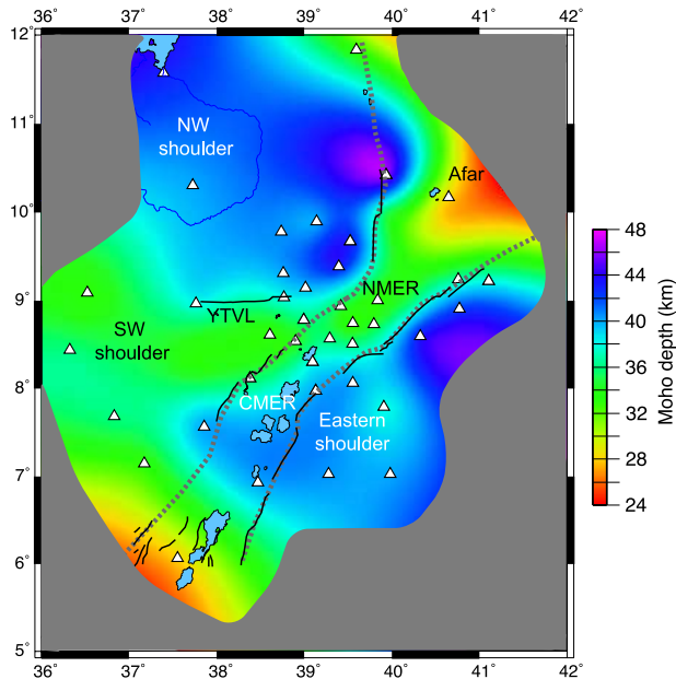
Figure 10. Contour map of Moho depth from our joint inversion results. The dashed gray lines show the rift outlines. Solid black lines are the rift border faults. White triangles are the stations we utilized from the EAGLE and EBSE networks. Crustal thickness beneath the rift shoulders is generally \sim 40 km, with the exception of the SW shoulder, which has a thickness of \sim 35 km. Crustal thickness within the NMER is \sim 35 km and within the CMER is 38–40 km (from this study and previous studies).
