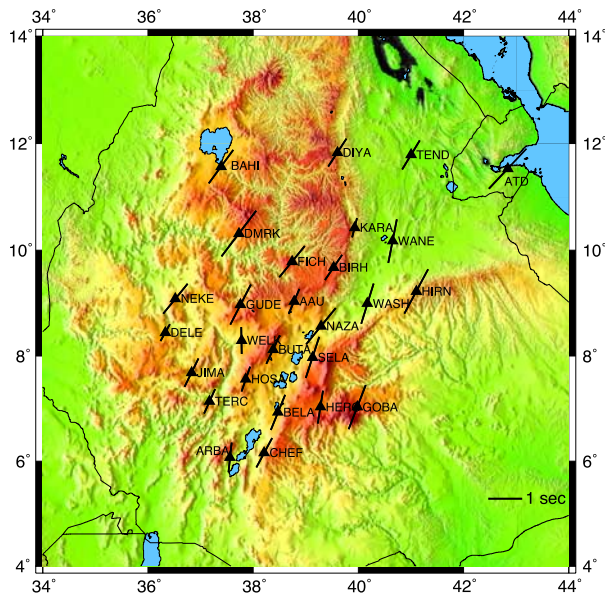
Figure 17. Shear wave splitting results across the MER and the Ethiopian Plateau modified from Gashawbeza et al. [2004]. Stations are represented by black triangles. The azimuth of the line at each station represents the azimuth of the fast direction of polarization of the shear wave. The length of the line is scaled according to the delay time between the arrivals in the fast and slow polarization directions, which is a measure of the integrated anisotropy below the station. Both the azimuth and the delay time remain relatively constant across the study area and are interpreted as reflecting the broad (~400-km-wide) distribution of melt not only beneath the rift but beneath the rift shoulders far from the surface structural expression of the rift.
